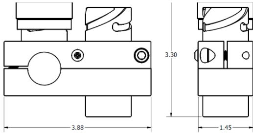
Handlebar Mounted Version
