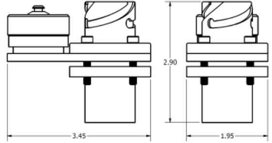
Panel Mount Version (1/4" Max Panel Thickness)
